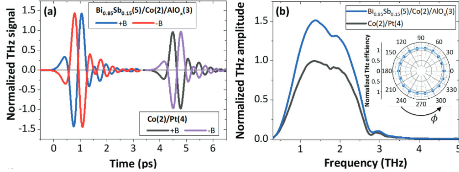
Figure 2.13: (a) THz emission signal in the time domain from \text{Bi}_{0.85}\text{Sb}_{0.15}(5 \text{ nm})/\text{Co}(2 \text{ nm})/\text{AlO}_x(3 \text{ nm}) in two directions of the in-plane saturating magnetic field ( \pm B ). (b) Spectral components of the THz emission from \text{Bi}_{0.85}\text{Sb}_{0.15}(5 \text{ nm})/\text{Co}(2 \text{ nm})/\text{AlO}_x(3 \text{ nm}) for +B. Adapted from [138].
