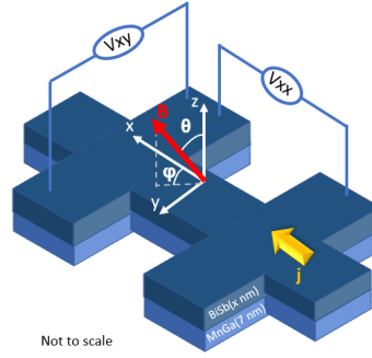
Figure 4.10: The geometry of a Hall bar for electrical measurements that involves injecting a current I (or current density \mathbf{j} ), in the +\mathbf{x} direction. It allows to measure both the longitudinal voltage V_{xx} and the transverse voltage V_{xy} , from which we can then deduce the longitudinal resistance R_{xx} and the transverse resistance R_{xy} . In addition, we can also apply an external magnetic field \mathbf{B} at angles (\theta, \varphi) . The thickness of the MnGa layer remains constant at 7 nm for all measurements, whereas the thickness of the BiSb layer will vary.
