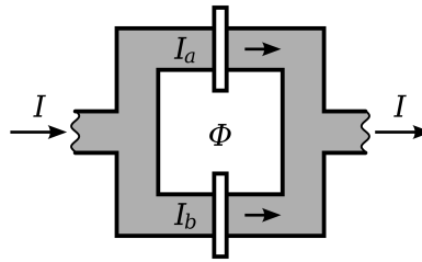
Figure 5.18: Schematic representation of a DC-SQUID device. The current I splits into the two paths with currents I_a and I_b . The barriers in each path are Josephson junctions. \Phi is the magnetic flux going through the superconducting loop.
