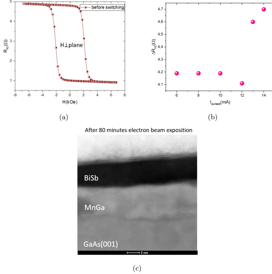
Figure 5.9: (a) The AHE measurements are done before each current pulse from 6 mA to 14 mA to monitor the change in resistance in the \text{Bi}_{0.90}\text{Sb}_{0.10}(9 \text{ nm})/\text{Mn}_{0.45}\text{Ga}_{0.55}(7 \text{ nm})/\text{GaAs}(001) system during the magnetization switching experiment. (b) The correspondent change in resistance as a function of the injected current pulses. (c) STEM measurements in BF mode of the \text{Bi}_{0.90}\text{Sb}_{0.10}(9 \text{ nm})/\text{Mn}_{0.45}\text{Ga}_{0.55}(7 \text{ nm})/\text{GaAs}(001) bi-layer after 80 minutes of electron beam exposition: the MnGa layer becomes amorphous that may result from the thermal instability. The BiSb layer remains crystalline.
