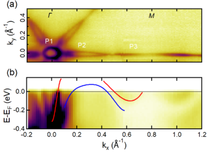
Figure 2.8: ARPES measurements for a 15 nm-thick \text{Bi}_{0.85}\text{Sb}_{0.15}/\text{Si}(111) thin film performed at room temperature with linearly vertical polarized light at 25.2 eV. (a) Recorded Fermi surface and (b) band structure along \bar{\Gamma M} . Red and blue lines correspond respectively to the two surface states: S_1 and S_2 . Adapted from [11].
