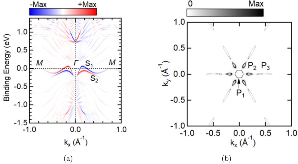
Figure 2.9: Tight binding calculations of the band structure of a 5 nm-thick \text{Bi}_{0.93}\text{Sb}_{0.07} (a) Electronic band structure along \bar{\Gamma M} showing two surface states: S_1 and S_2 . (b) Fermi surface showing three electron (P1, P3) and hole pockets (P2). Adapted from [11].
