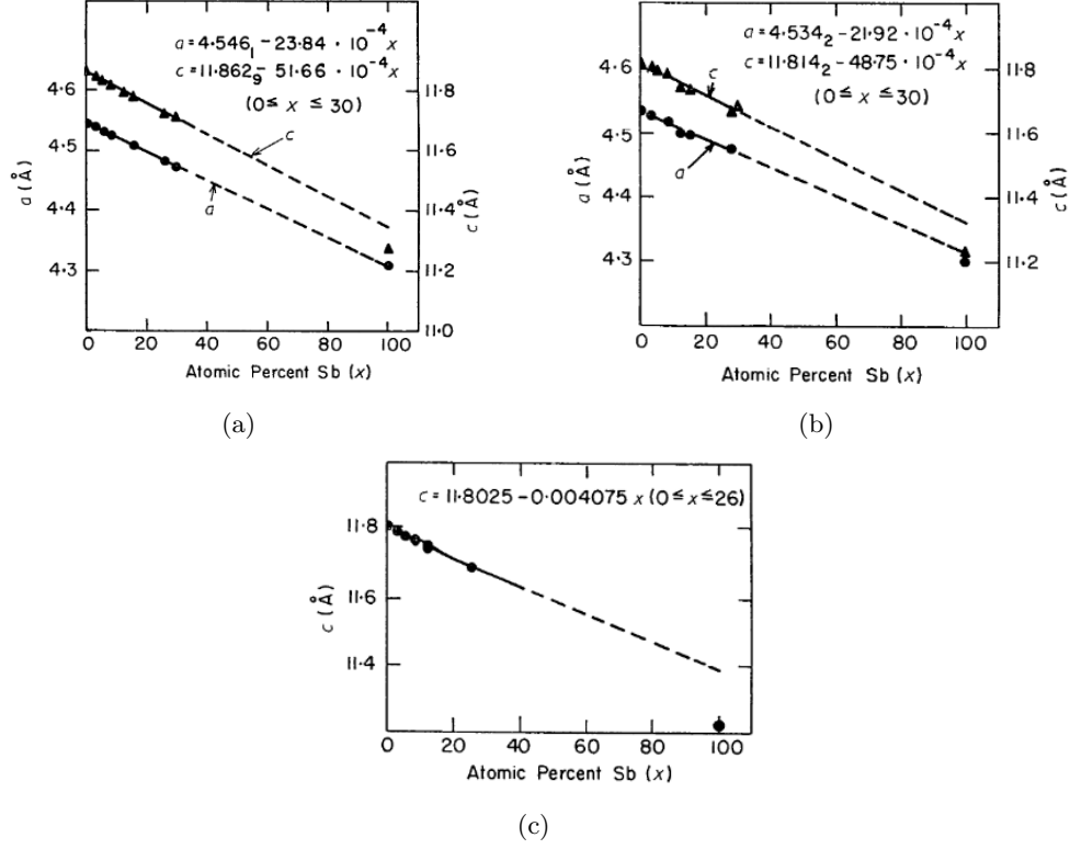
Figure 2.6: Hexagonal lattice constants of Bi-Sb alloys at: (a) 298±3K, (b) 78K, (c) 4.2K. Adapted from [29].
