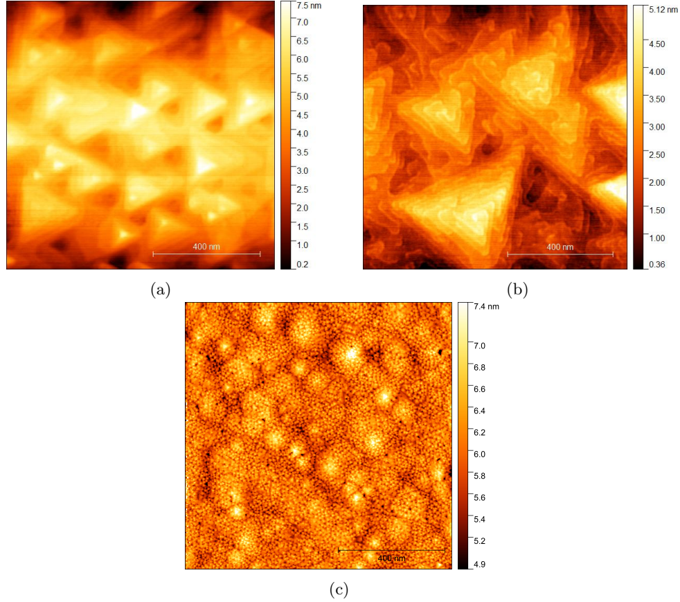
Figure 3.8: AFM images of: (a) Bi/InSb(111)B, (b) \text{Bi}_{0.82}\text{Sb}_{0.18}/\text{InSb}(111)\text{B} , (c) \text{Bi}_{0.82}\text{Sb}_{0.18}/\text{InSb}(111)\text{B} with chemical etching. The scan field is 1 \times 1 \mu\text{m}^2 .
