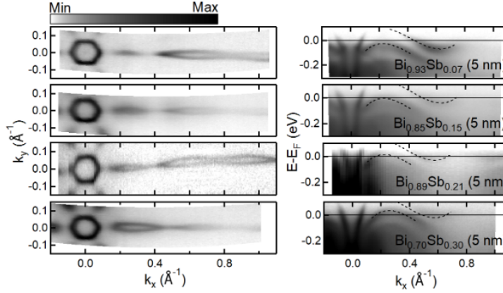
Figure 2.10: ARPES measurements for \text{Bi}_{1-x}\text{Sb}_x (5 nm) as a function of various concentrations of Sb x : 7%, 15%, 21% and 30%. Left panel: Fermi surfaces along the \bar{\Gamma}M direction. Right panel: Corresponding cross sections. Adapted from [11].
