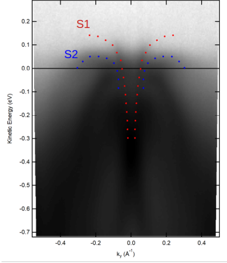
Figure 4.5: Band dispersion measured by ARPES along the \bar{\Gamma}\bar{M} direction at room temperature on Sample 1 using a photon energy of 20 eV. The two S_1 and S_2 surface states are highlighted by red and blue dashed lines, respectively.
