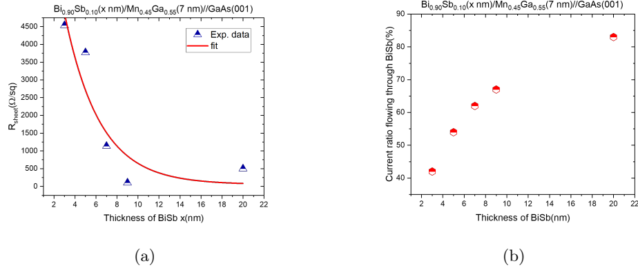
Figure 4.12: (a) Sheet resistance of the \text{Bi}_{0.90}\text{Sb}_{0.10}(x \text{ nm})/\text{Mn}_{0.45}\text{Ga}_{0.55}(7 \text{ nm})/\text{GaAs}(001) as a function of the thickness of the BiSb layer x . (b) Current ratio distribution flowing through the \text{BiSb}(x \text{ nm}) layer in the \text{Bi}_{0.90}\text{Sb}_{0.10}(x \text{ nm})/\text{Mn}_{0.45}\text{Ga}_{0.55}(7 \text{ nm})/\text{GaAs}(001) system.
