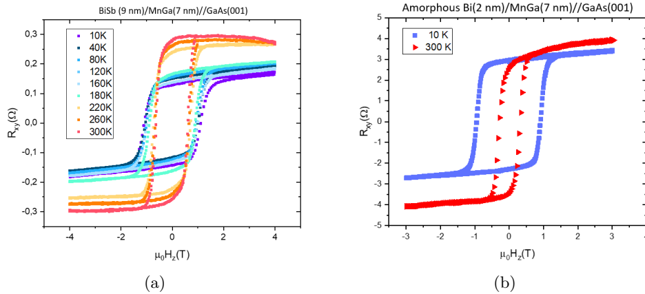
Figure 4.14: AHE hysteresis cycles at different temperatures with the magnetic field applied out of plane \mathbf{H} = H_z \mathbf{z} for the (a) \text{Bi}_{0.90}\text{Sb}_{0.10}(9\text{ nm})/\text{Mn}_{0.45}\text{Ga}_{0.55}(7\text{ nm}) bilayer and (b) \text{Mn}_{0.45}\text{Ga}_{0.55}(7\text{ nm}) single layer capped with a 2 nm amorphous Bi layer.
