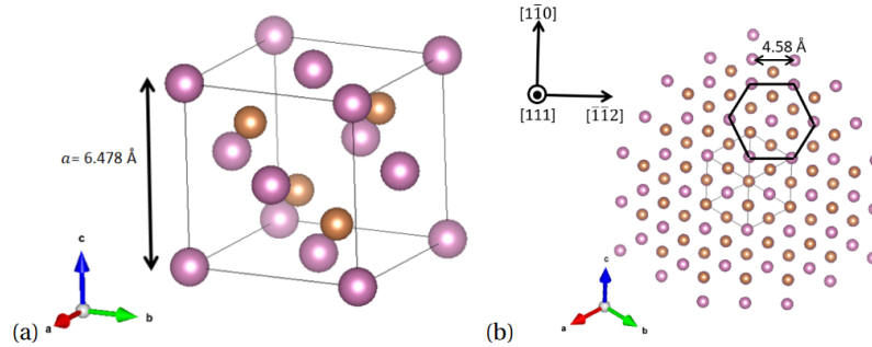
Figure 3.3: (a) Unit cell structure of \text{InSb} . Purple and yellow spheres represent In and Sb atoms, respectively. (b) (111) plan of \text{InSb} . Extracted from [10].
