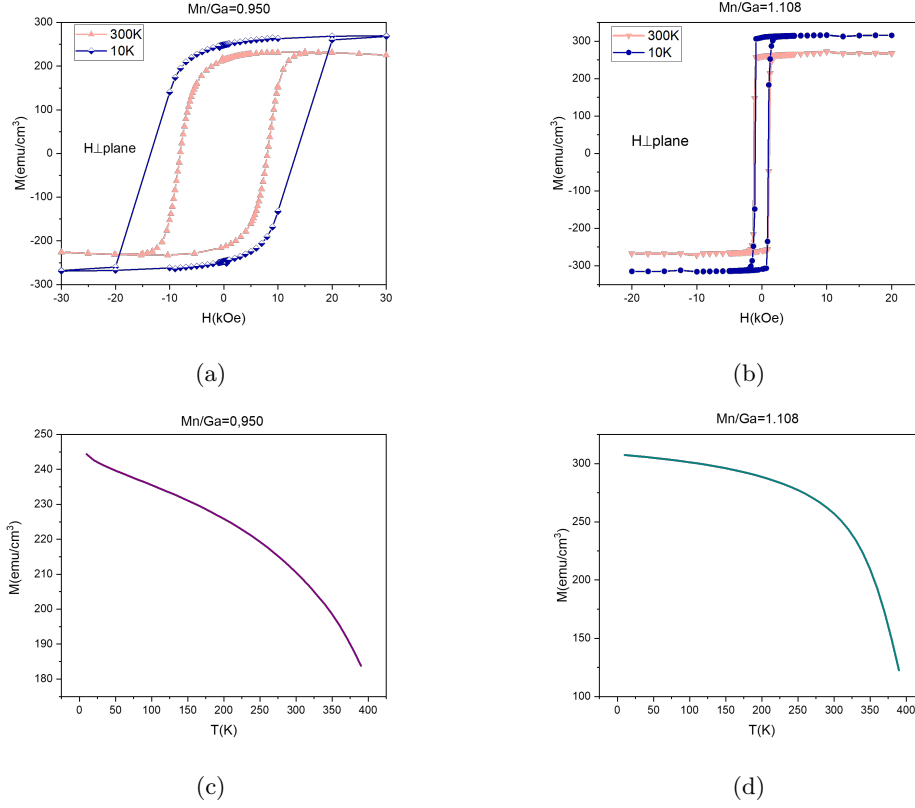
Figure 3.19: SQUID data of MnGa//GaAs(001) thin layers with the external field applied out of plane: (a) Hysteresis cycle for Mn/Ga ratio = 0.950 at 300K (in pink) and at 10K (in blue). (b) Hysteresis cycle for Mn/Ga ratio = 1.108 at 300K (in pink) and at 10K (in blue). Magnetization M as a function of temperature T : (c) for Mn/Ga ratio = 0.950, (d) for Mn/Ga ratio = 1.108.
