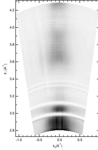
Figure 4.6: (k_x, k_y) Fermi surface recorded on Sample 1, calculated using V_0=10 eV.
